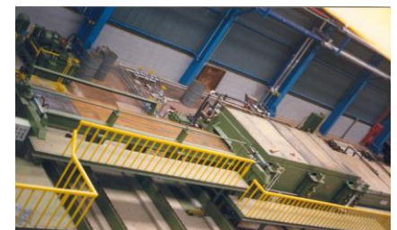
72" x .500" x 60,000# Pro-Eco Pickle Line, (3) Tank System
